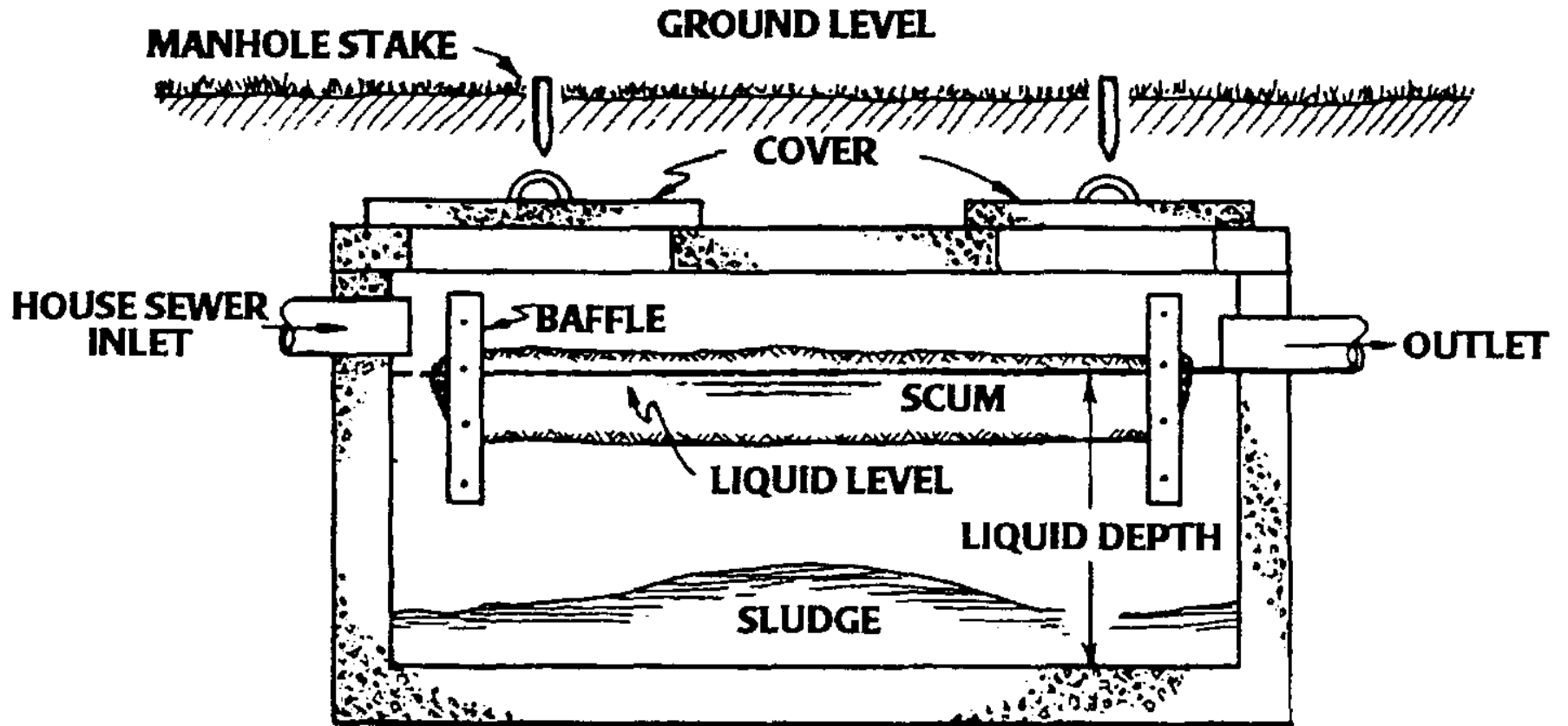
CROSS SECTION OF A TYPICAL CONCRETE SEPTIC TANK
